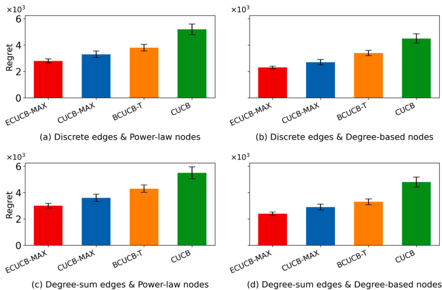
Fig. I.11. Regret@ T=1500 of algorithms under extended experimental settings.
