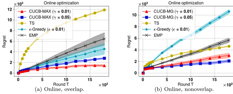
Fig. 6. Cumulative regret for online algorithms when B = 3000 .
