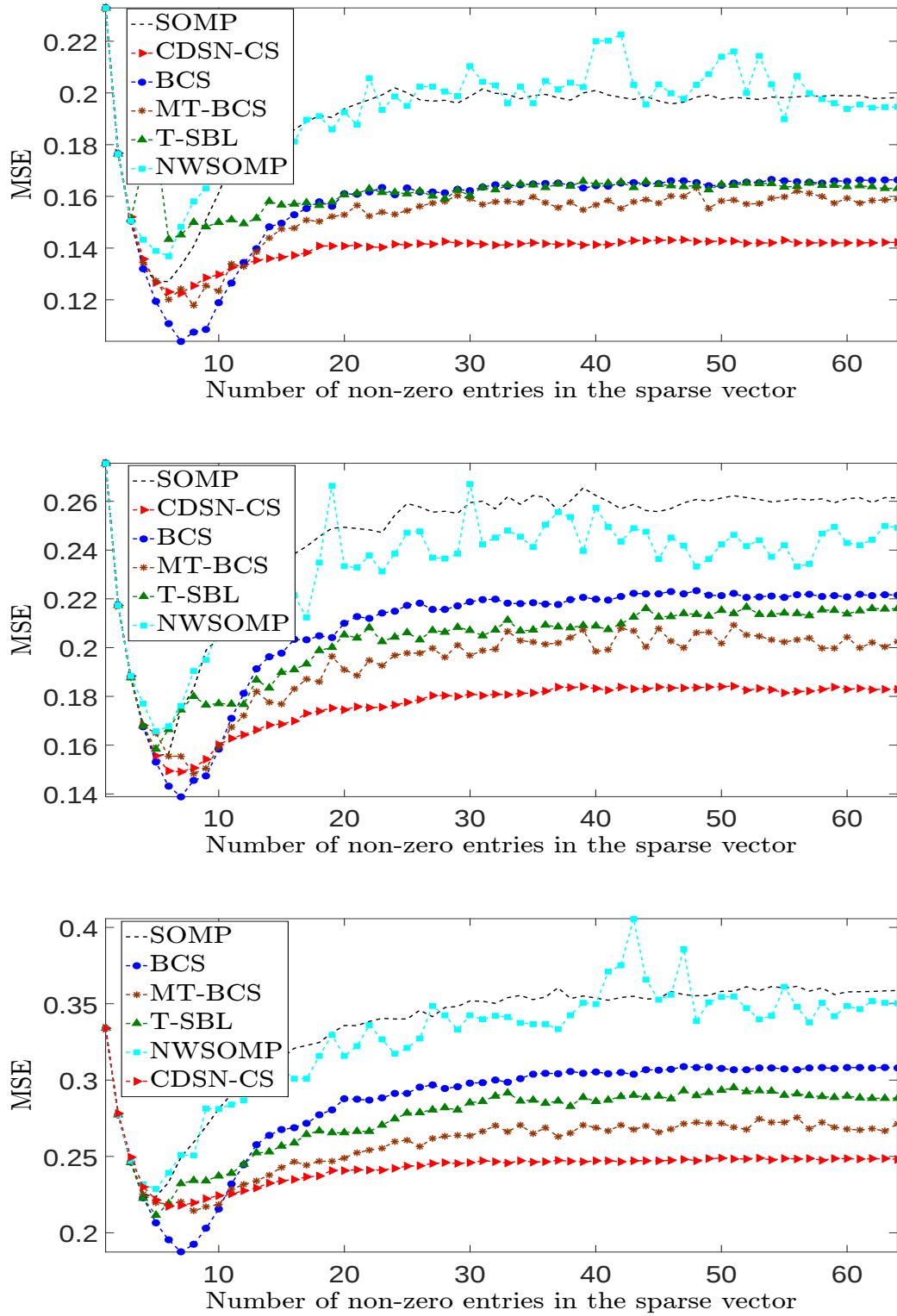
Figure 4.20: Comparison of different MMV reconstruction algorithms performance for the natural image dataset using Wavelet transform. Image classes from top to bottom are buildings, cows and flowers respectively.
