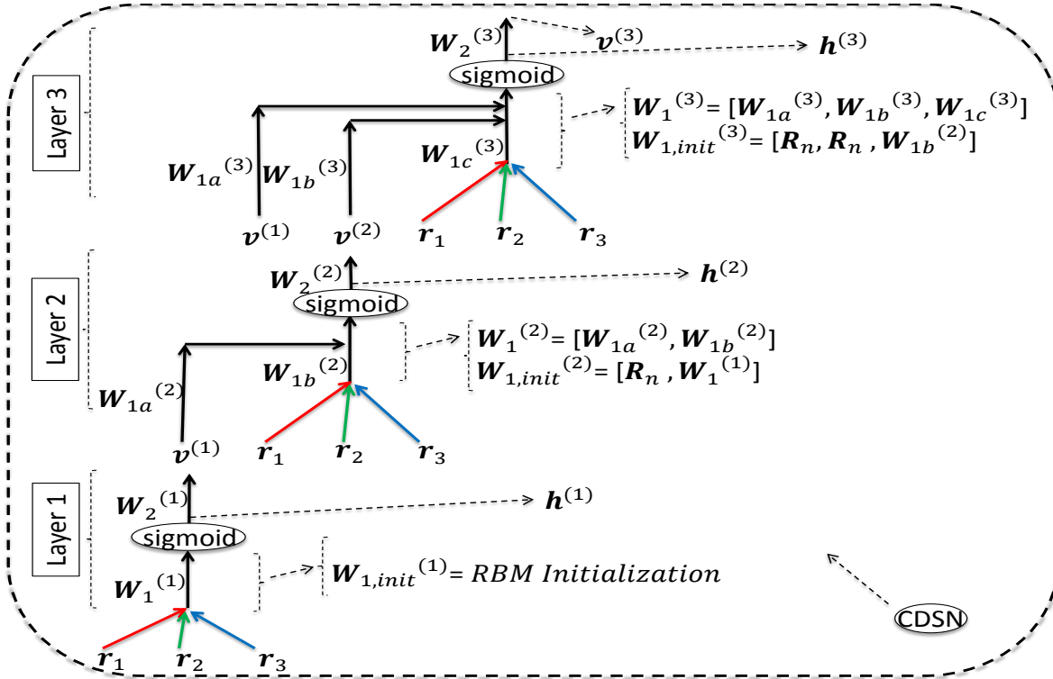
(b) Block diagram of the convolutional deep stacking network with 3 layers. This diagram shows CDSN for channel 2 in Fig. 4.16(a), and R_n denotes a random matrix.
