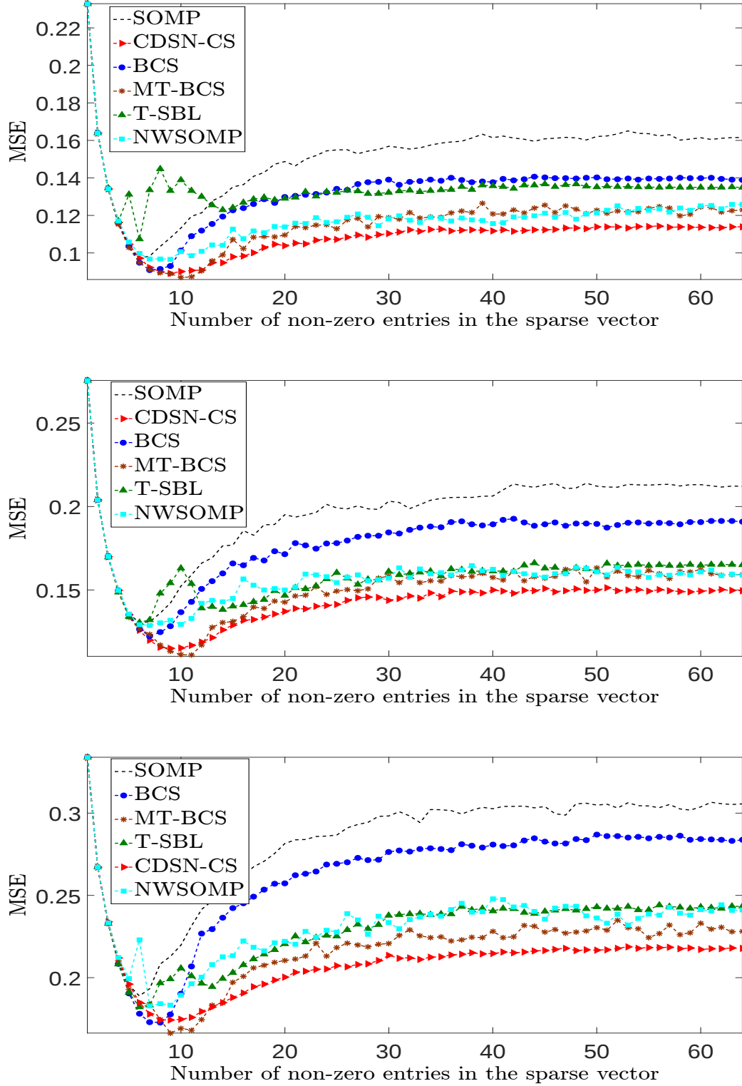
Figure 4.19: Comparison of different MMV reconstruction algorithms performance for the natural image dataset using DCT transform. Image classes from top to bottom are buildings, cows and flowers respectively.
