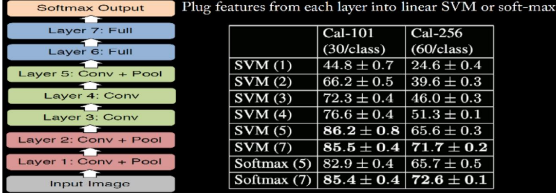
Figure 1.2: Importance of depth (Figure from [40]).
