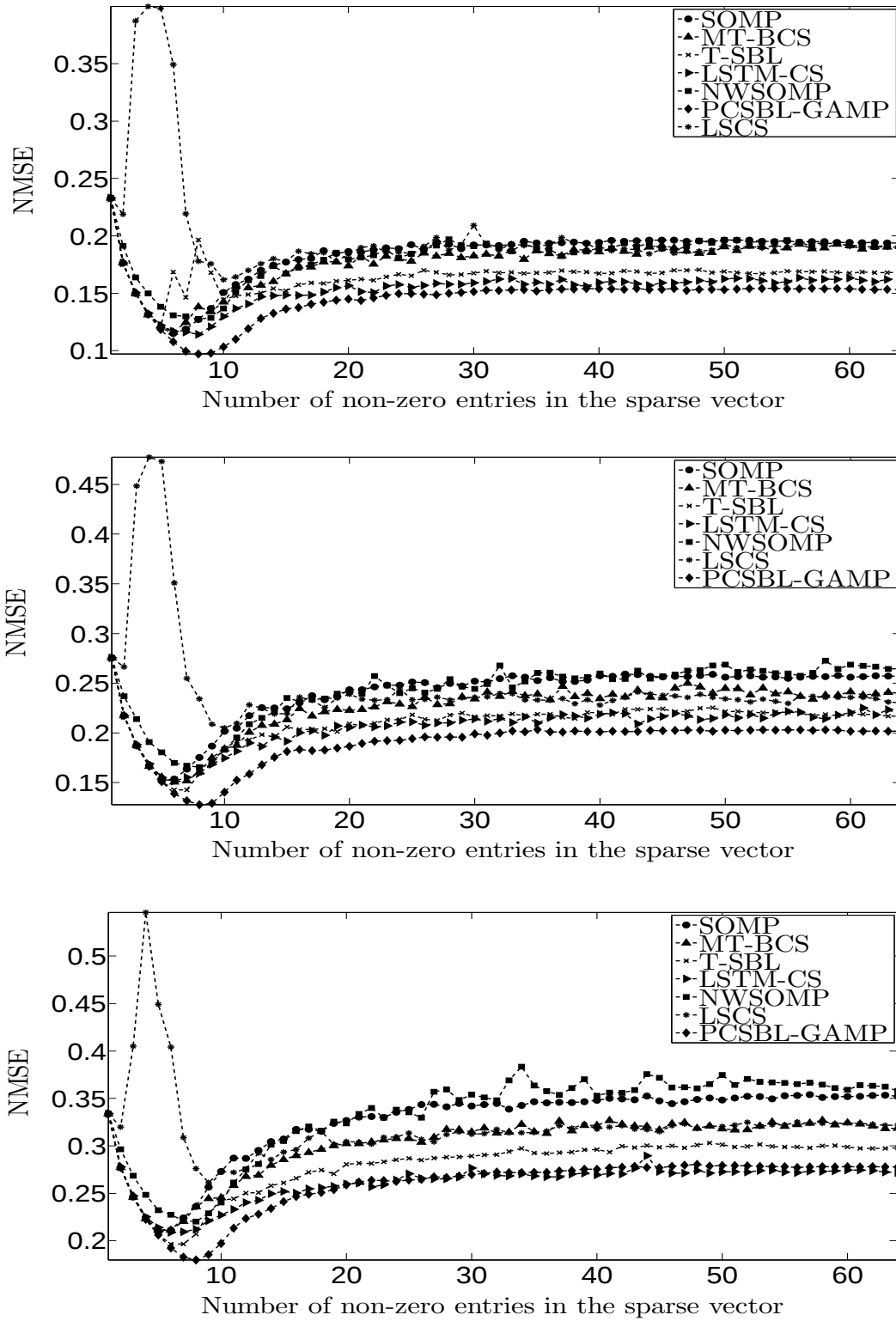
Figure 4.12: Comparison of different MMV reconstruction algorithms for natural image dataset using Wavelet transform and just one layer for LSTM model in LSTM-CS. Image classes from top to bottom respectively: buildings, cows and flowers.
