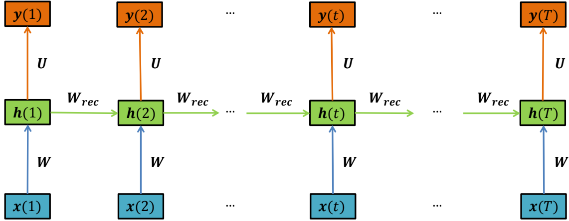
Figure 1.5: One layer RNN unfolded over time.
