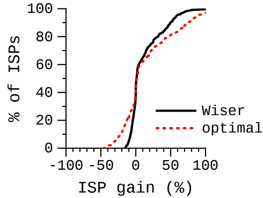
Figure 5.4: The CDF of gain for ISPs in individual bilateral relationships with Wiser and optimal . The gain is measured as the average reduction in distance relative to anarchy . There are two points in each CDF for each pair of ISPs.
