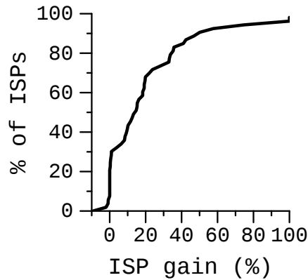
Figure 5.3: The CDF of gain for individual ISPs with Wiser, measured as the reduction in average distance relative to anarchy .
