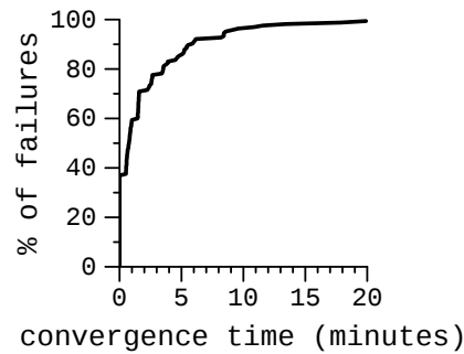
Figure 5.18: The CDF of convergence time of Wiser with load-sensitive agnostic costs.
