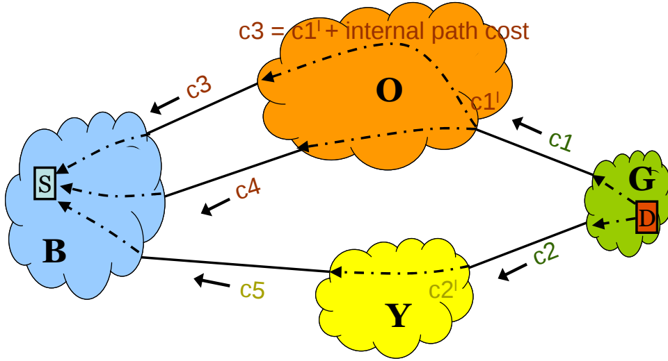
Figure 4.5: Wiser in the case of multiple ISPs. Downstream ISPs announce agnostic costs to upstream ISPs. ISPs normalize incoming agnostic costs and propagate them after adding their internal path costs. To select paths (not shown in the figure), the source considers both the local and received agnostic costs.
