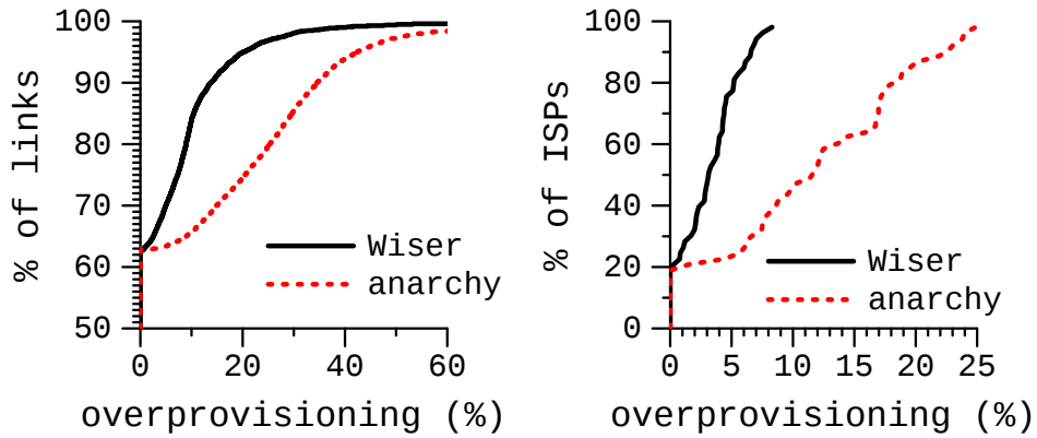
Figure 5.7: Overprovisioning required with Wiser and anarchy to deal with tier-1 inter-connection failures. Left : The CDF of link-level overprovisioning. Right : The CDF of ISP-level overprovisioning. Note that the x - and y -axis ranges are different for the two graphs.
