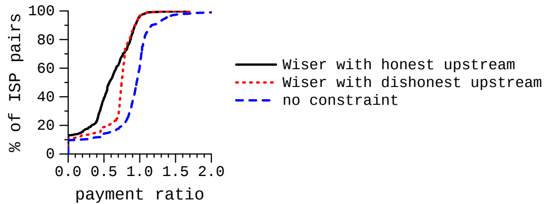
Figure 5.23: The CDFs of payment ratio with Wiser, both when the upstream ISP is honest and when it is dishonest within the bounds of Wiser, and in a scenario where the cheating is not constrained.
