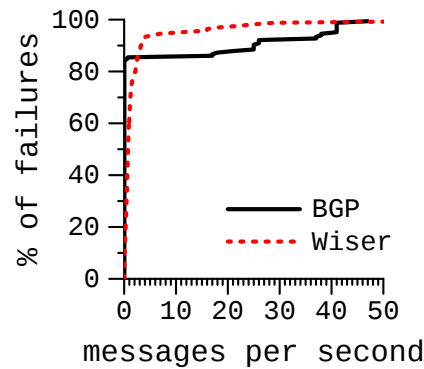
Figure 5.19: The CDF of maximum rate of routing messages for Wiser with load-sensitive agnostic costs. The curve for BGP is reproduced from Figure 5.17.
