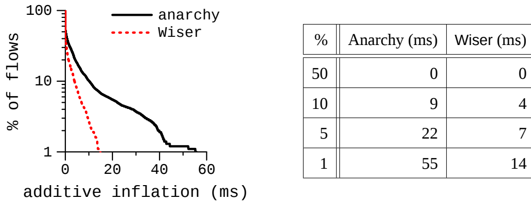
Figure 5.2: Additive inflation in path length with anarchy and Wiser relative to optimal . The graphs plots the CCDF of inflation on a log scale. The table summarizes the graph.
