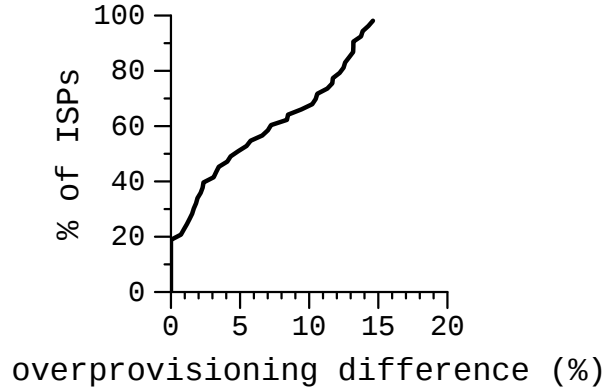
Figure 5.9: The CDF of the difference in overprovisioning between anarchy and Wiser for individual ISPs.
