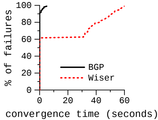
Figure 5.16: The CDF of convergence time of BGP and Wiser with load-insensitive agnostic costs.
