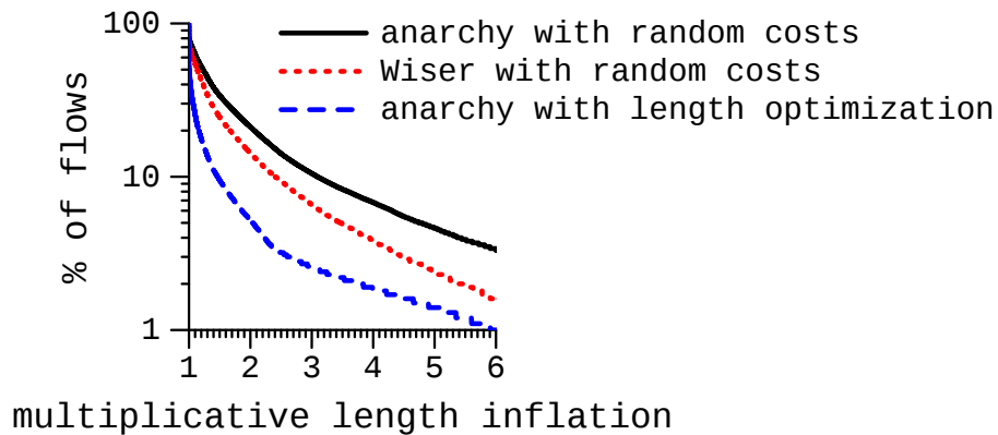
Figure 5.14: The CCDF of multiplicative inflation in path length with different routing methods. The inflation is measured relative to optimal that minimizes path length.
