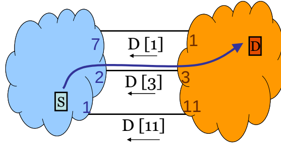
Figure 4.2: Wiser in the two ISP case. The numbers inside the upstream ISP (on the left) represent its agnostic costs of carrying traffic between S and the corresponding interconnection, and those inside the downstream ISP represent its agnostic costs of carrying traffic between the interconnections and D . With Wiser, the downstream ISP discloses its agnostic costs to the upstream ISP, and the upstream ISP selects an interconnection based on both its own and the downstream ISP's costs.
