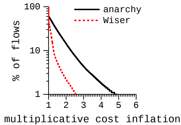
Figure 5.12: Efficiency of Wiser and anarchy with heterogeneous ISP objectives. The graph plots the CCDF of multiplicative inflation in cost relative to the chosen Pareto-optimal routing pattern.
