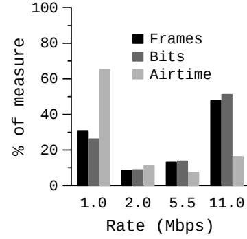
Figure 6: Relative prevalence of transmission rates.
