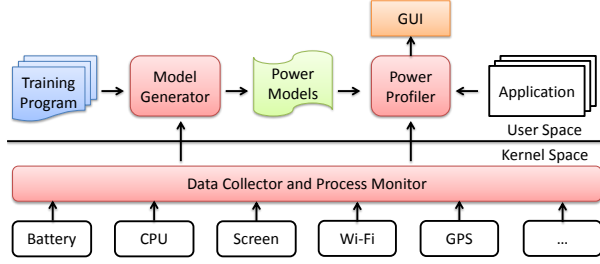
Figure 5: System architecture based on V-edge.
