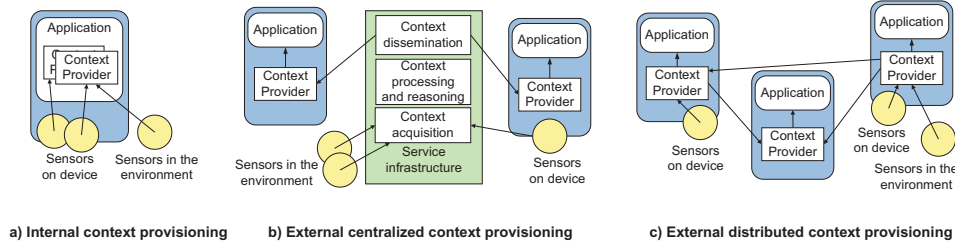
Fig. 1. Context provisioning strategies
