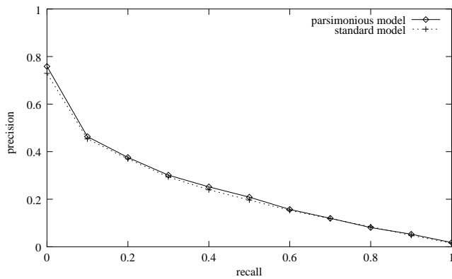
Figure 4: Recall-precision graphs of language models on the ad hoc task
