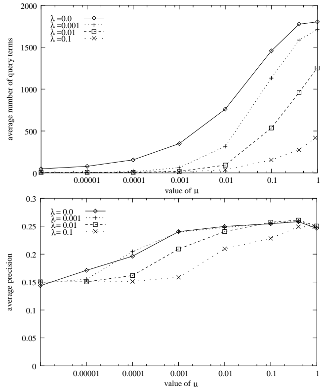
Figure 3: Relevance models: \mu vs. 1) average number of query terms, 2) average precision
