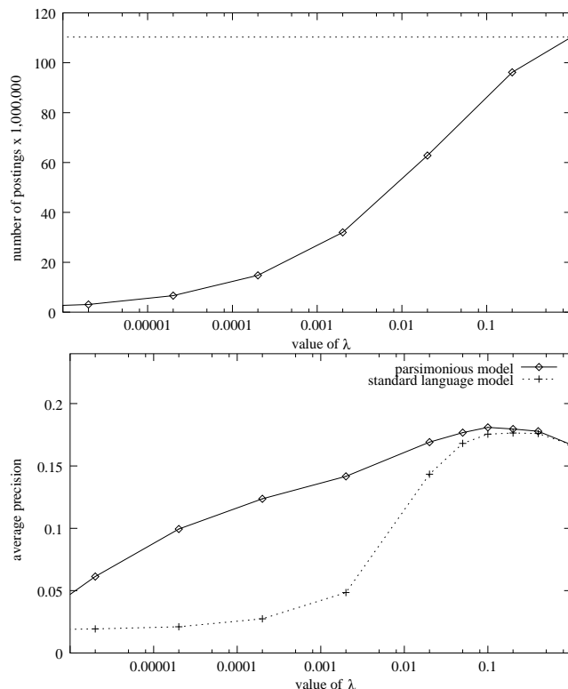
Figure 1: Document models: \lambda vs. a) number of postings b) average precision
