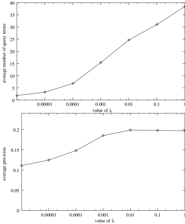
Figure 2: Query models: \lambda vs. 1) average number of query terms, 2) average precision
