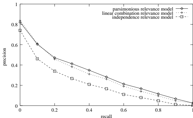
Figure 5: Recall precision graphs of relevance models on the routing task
