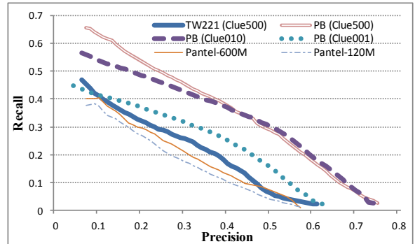
Figure 1. Precision and recall of various approaches (query set: WikiGold)
