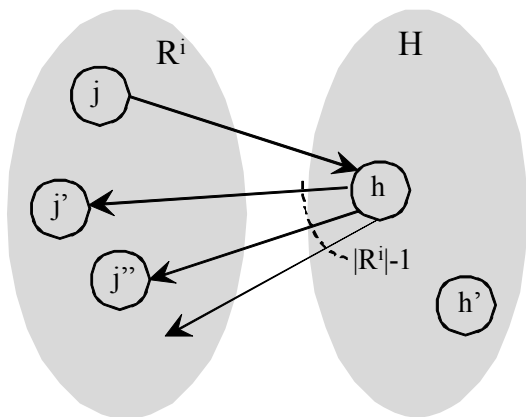
Fig. 3. Modifying coding solution using replication at each h \in H to all j \in R^i .
