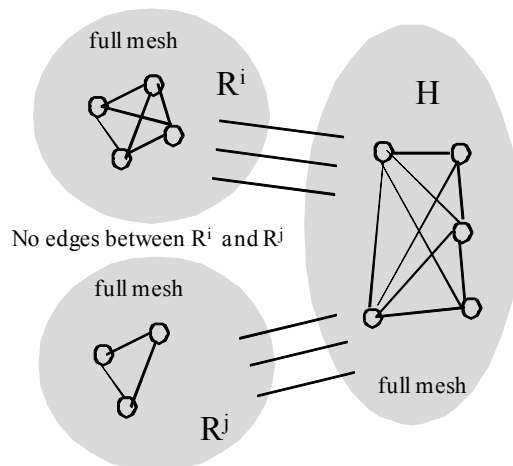
Fig. 2. Communication graph for the scenario in Theorem 2.
