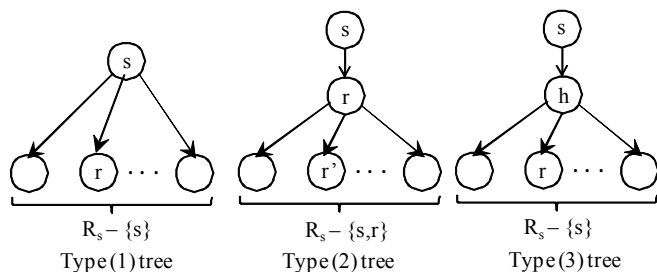
Fig. 1. Different types of Mutualcast trees.
