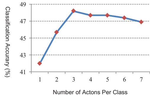
Figure 4. The classification performance w.r.t. different number of actions (i.e., parameter K ) learned in the second layer. The results are obtained with the MBH feature on HMDB51 dataset.
