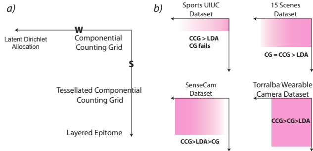
Figure 7. a) CCG Spectrum b) Performance across the spectrum on the database used in the experiments.
