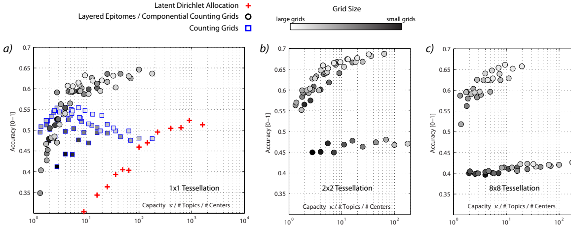
Figure 4. Results on SenseCam (Mean results over 5 repetitions). As the same \kappa can be obtained with different choice of \mathbf{E} and \mathbf{W} , multiple results may be reported for the some values of \kappa . For (Componential) Counting Grids, we colored the markers based on the size of \mathbf{E} . a) Single Bag model and comparison with [4] and [7]. b) Moderate Tesselation results c) Fine Tesselation results.
