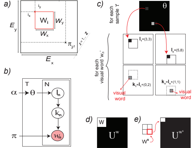
Figure 3. a) Counting Grid geometry. b) Componential Counting Grid/Layered Epitome generative model. c) CCGs generative process. d) Illustration of U^W ; e) Illustration of U^{W^s} in the case of a S = 2 \times 2 .
