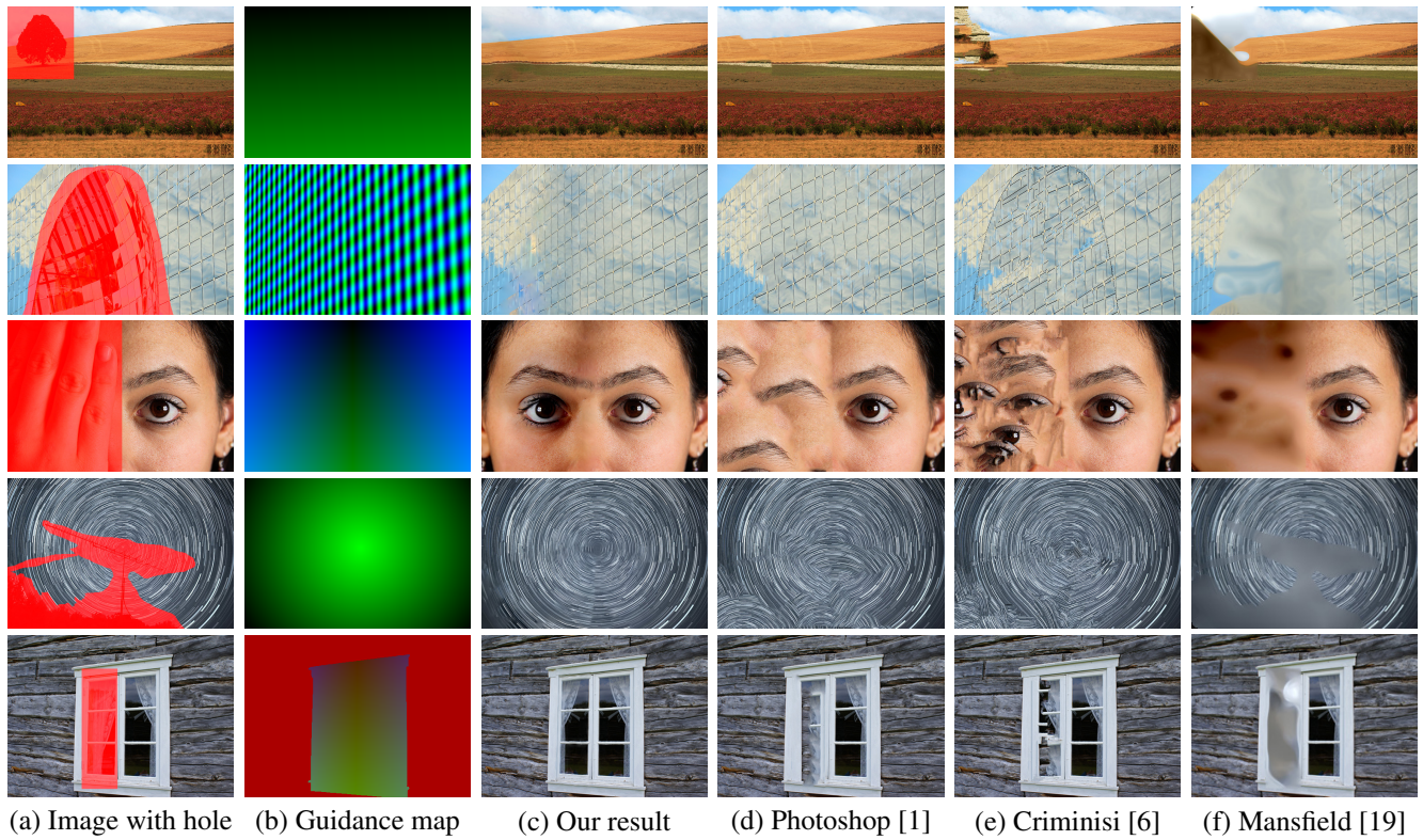
Figure 10. Comparisons to unguided algorithms. Completing these images without guidance is hard. From top to bottom: ramp, translational symmetry, reflective symmetry, rotational symmetry, and reflective symmetry on planar surface. More examples are shown in the supplementary file.
