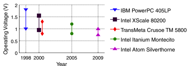
Figure 1. Operating voltage ranges
