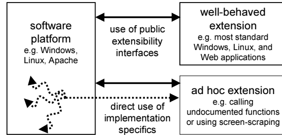
Figure 1. Well-behaved extensions interact with their platform via a public interface, whereas ad hoc extensions directly depend upon or manipulate the implementation details of their platform.
