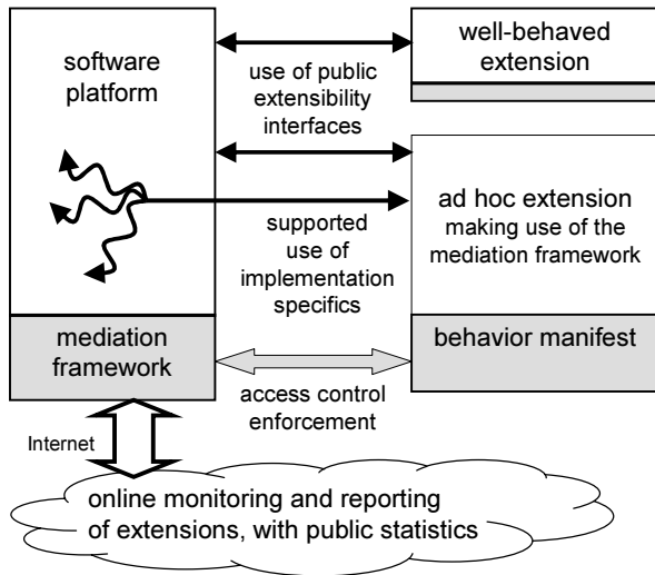
Figure 2. Our proposed architecture for making ad hoc extensions more dependable through the use of a mediation framework, the gathering and publication of online monitoring data, and behavior manifests that accompany extensions.
